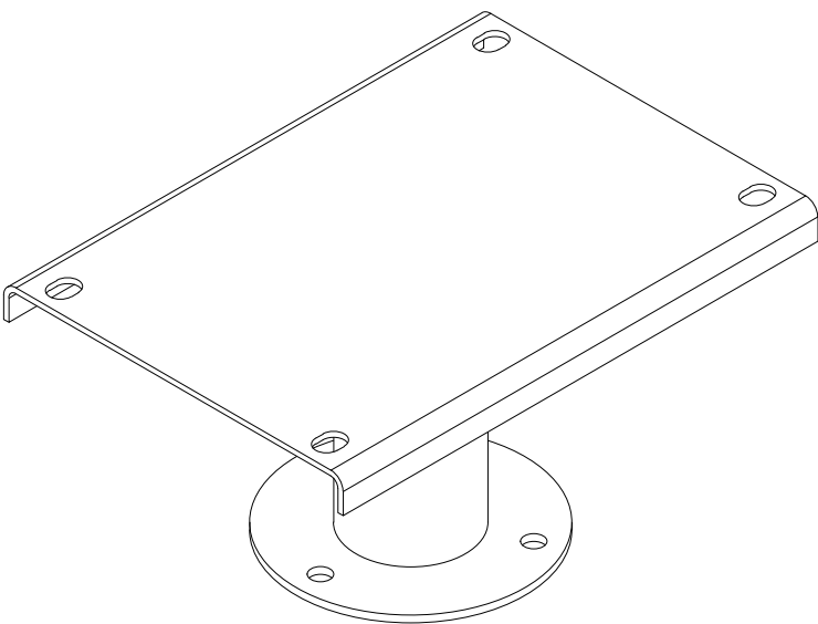
ISO VIEW
